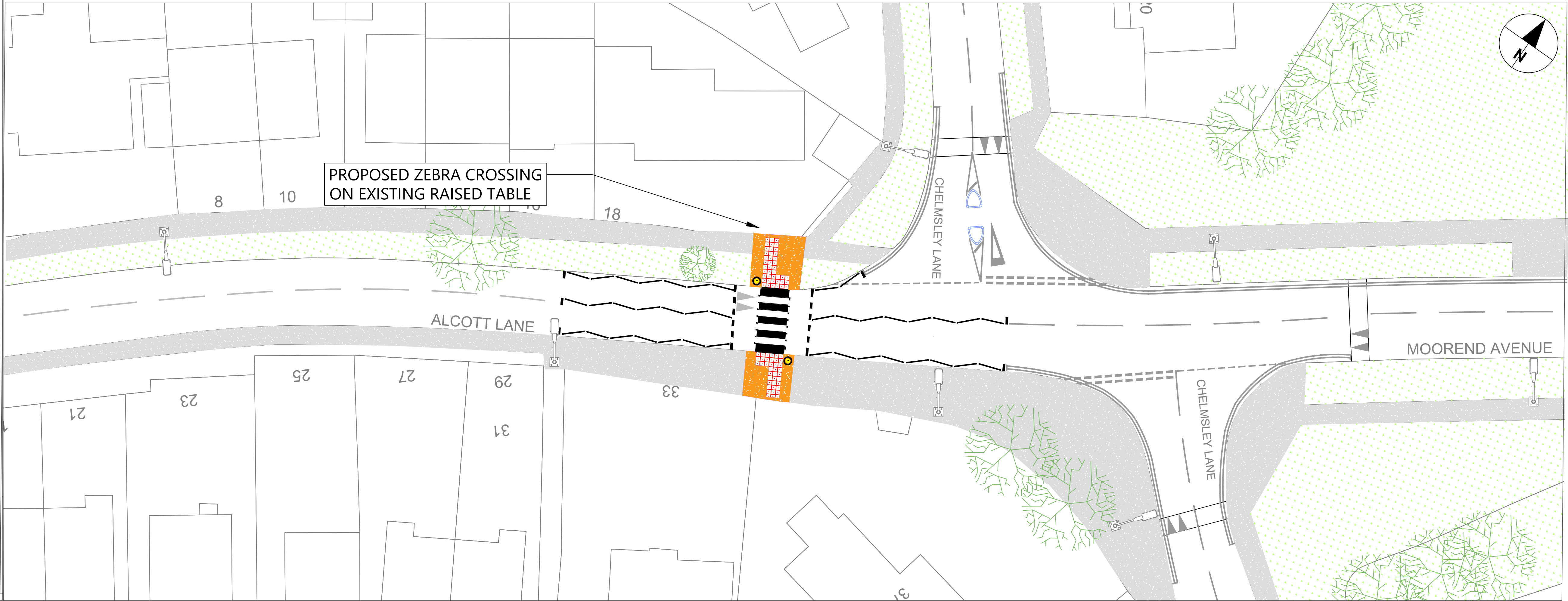
DETAILED LAYOUT SCALE (1:200)
