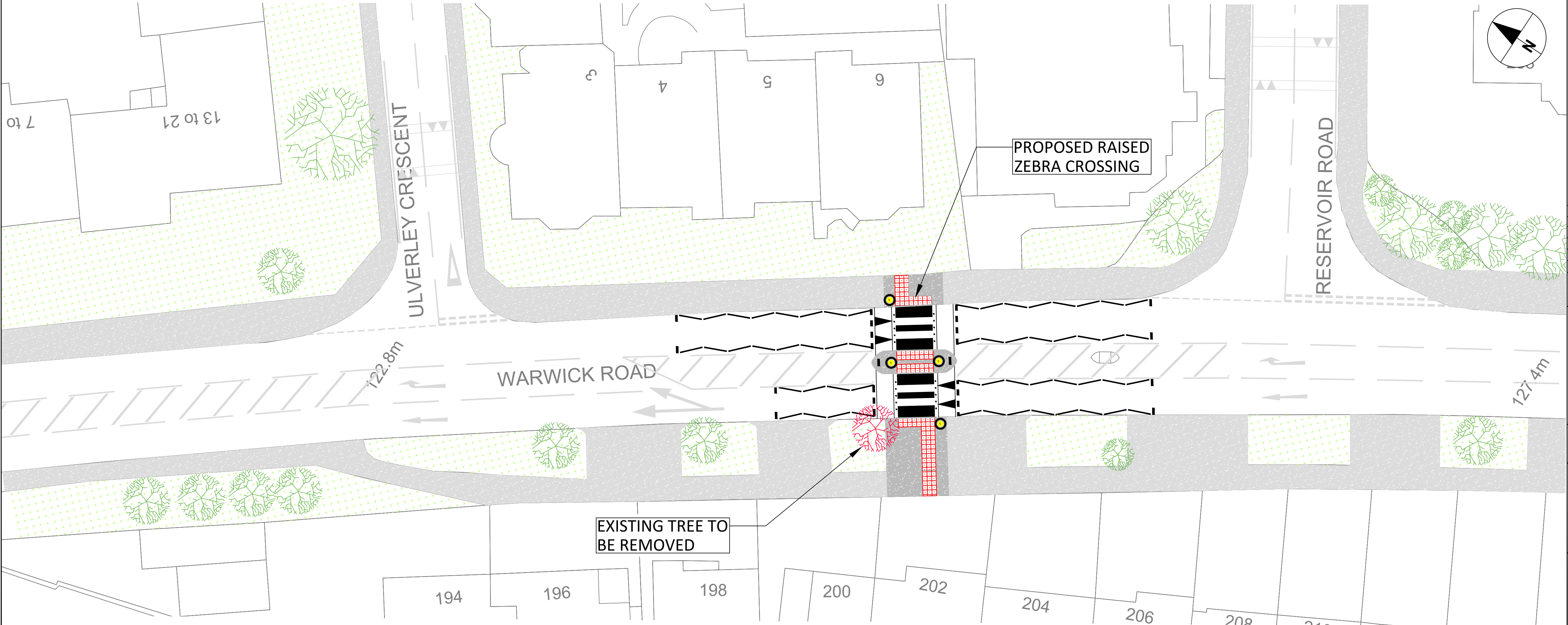
DETAILED PLAN (SCALE 1:200)
