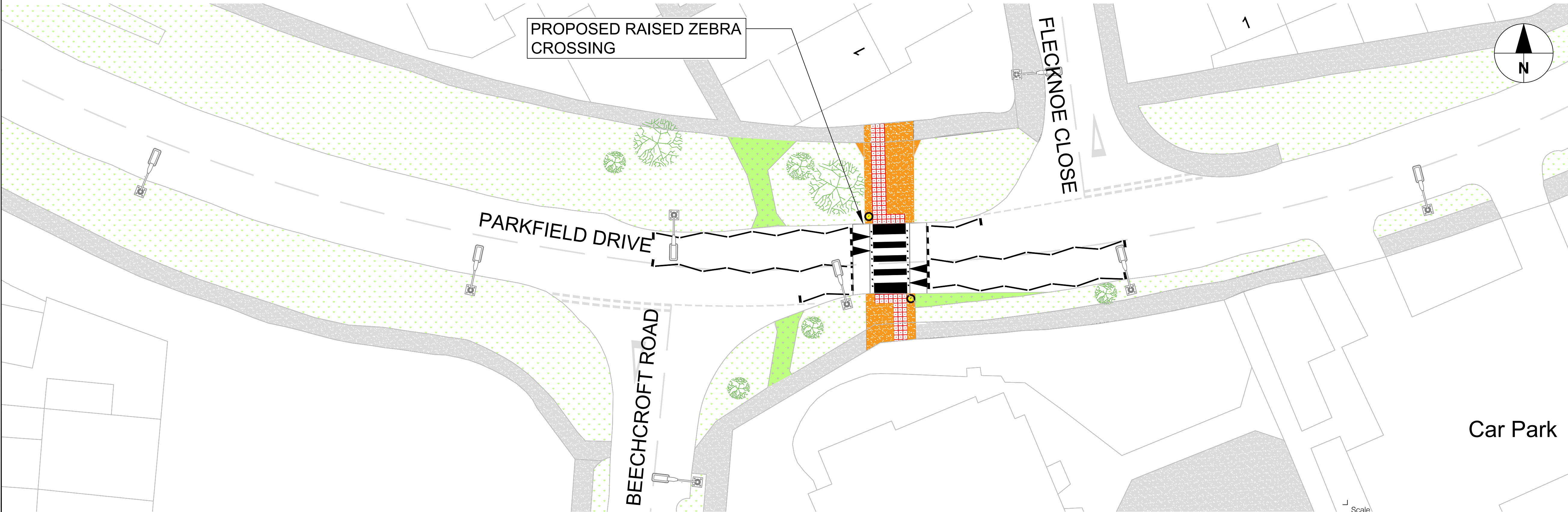
DETAILED LAYOUT (SCALE 1:200)
