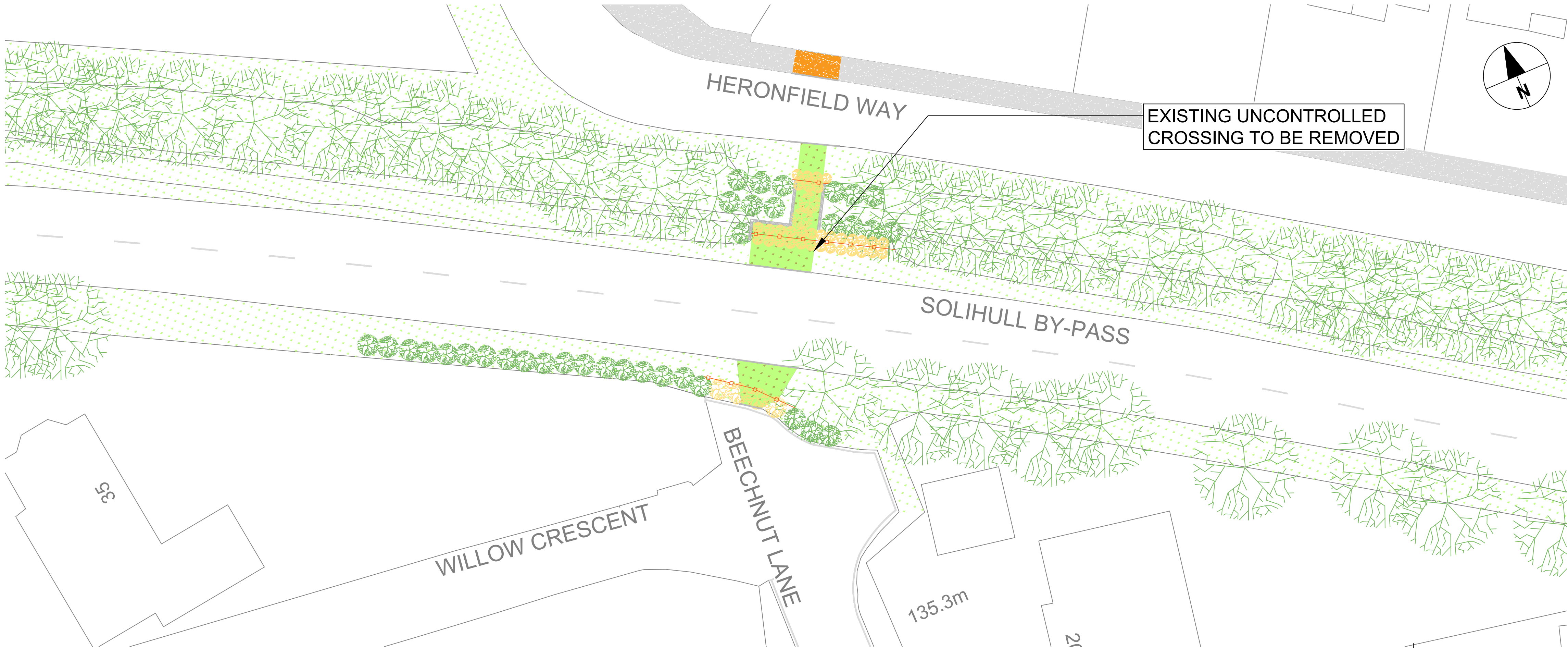
DETAILED PLAN (SCALE 1:200)
