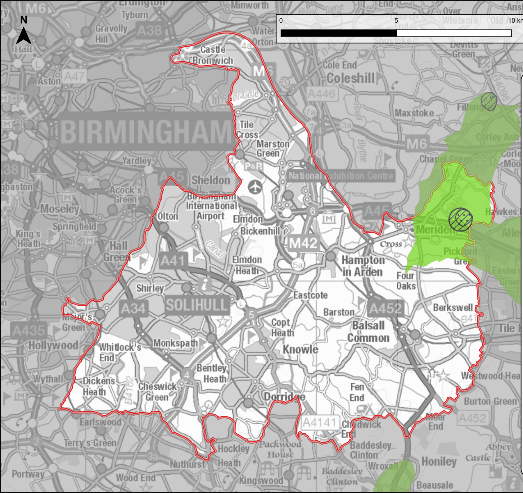
Solihull Groundwater Source Protection Zones
