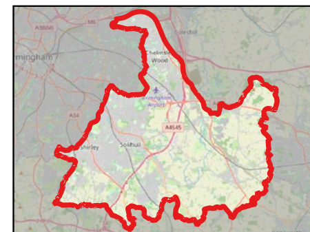
Solihull Groundwater Source Protection Zones
