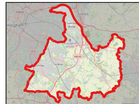
Solihull Superficial Geology
