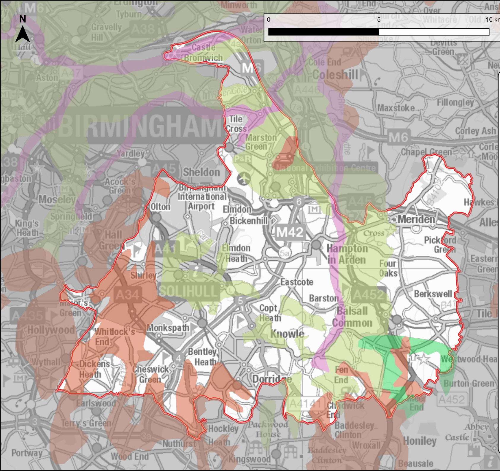
Solihull Superficial Geology
